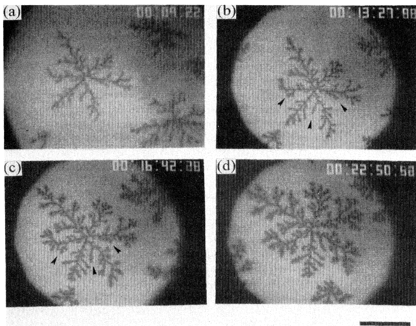
FIG. 6. When the LC domains of compound B were left on air-water interface for some time, the whole pattern shrank under the influence of surface tension. Some minor branches disappeared and only backbones were left (a). It is shown in these micrographs that shrinking LC domain may also grow under continuous illumination. Those branches marked by the arrows grew very slowly comparing to the other branches. This effect is the typical feature of diffusion-limited growth. On the upper right corners of (a)–(d), the first three codes in the timer represent hours, minutes, and seconds, respectively. The bar represents 50 \mu\text{m} .
