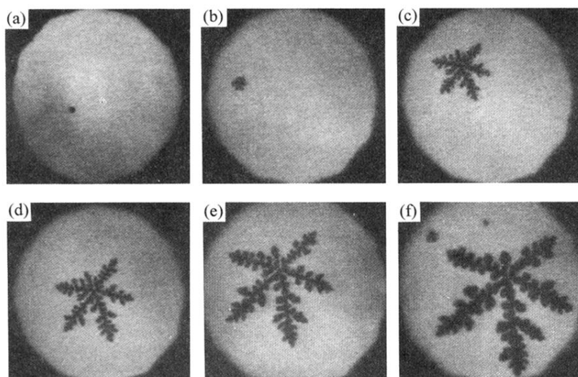
FIG. 3. The successive micrographs to show the illumination-related nucleation process of LC domains of compound A . Initially an area free of any LC domains was selected under the microscope. By illuminating this area continuously, a LC domain was nucleated (a). Continuous illumination made the domain grow. After a long time illumination, new generation of LC domains was induced, as shown in (f). The bar represents 100 \mu\text{m} .
