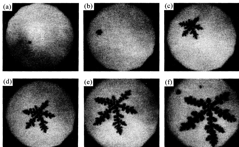
FIG. 3. The successive micrographs to show the illumination-related nucleation process of LC domains of compound A. Initially an area free of any LC domains was selected under the microscope. By illuminating this area continuously, a LC domain was nucleated (a). Continuous illumination made the domain grow. After a long time illumination, new generation of LC domains was induced, as shown in (f). The bar represents 100 \mu\text{m} .
